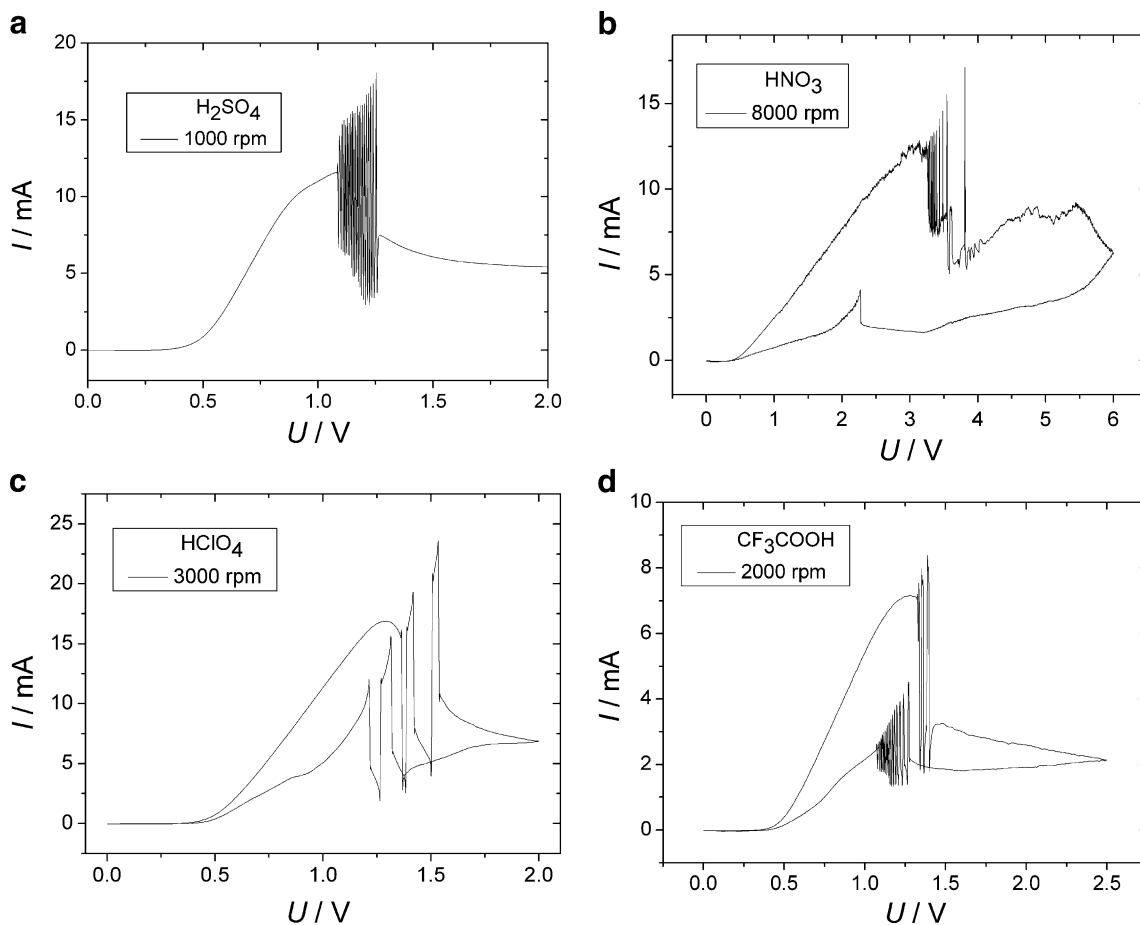
Fig. 8 Exemplary voltammetric curves of electrodisolution of rotating vanadium electrode (1-mm-diameter vanadium wire, embedded in Teflon) in various acidic media. Temperature T=0\text{ }^{\circ}\text{C} , scan rate
